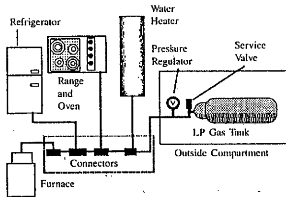
Typical LP Gas System
